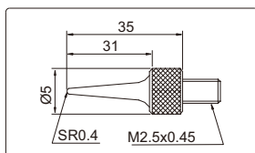
针型测针
